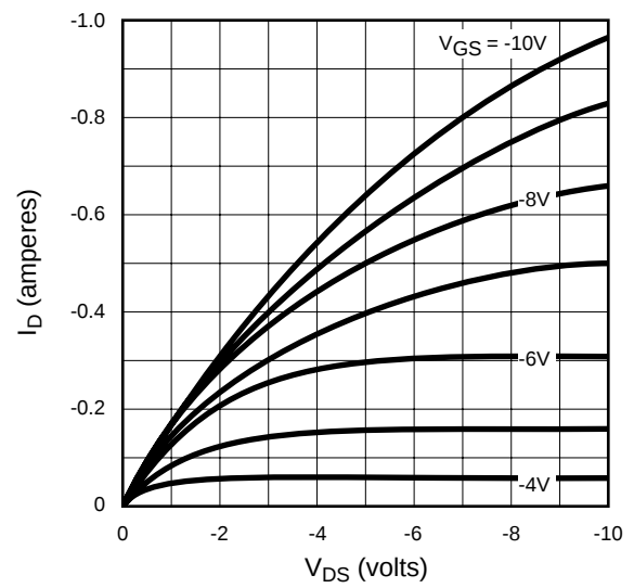
Saturation Characteristics
